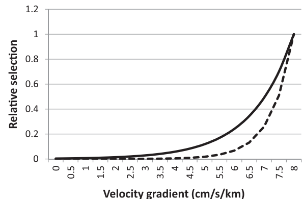
Fig. 7. Relative selection within the central Chukchi as a function of current gradient while controlling for the effects of salinity (solid line) or temperature (dashed line).
